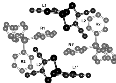
Fig. 1 The embrace between a pair of [Ph 4 P] + ions (light tones) and a pair of [Zn(mnt) 2 ] 2- ions (dark tones) in 1 . The four offset-face-to-face interactions in this centrosymmetric motif are L1...R1, L2...R2', L1'...R1' and L2'...R2.
