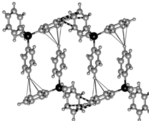
Fig. 7 Part of the column of [\text{MePh}_3\text{P}]^+ cations in PMPESEN. The stack of OFF motifs in the centre is formed by a stacking of P4PE secondary motifs comprising two VF (thin lines) and one OFF between a pair of cations. In addition there are EF motifs (candy-stripes) between contiguous P4PEs. The methyl groups are not involved.
