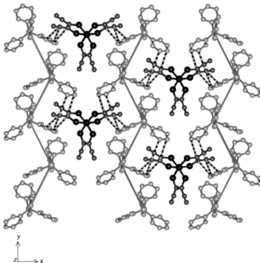
Fig. 12 The layer in [\text{Ph}_4\text{P}]_2[\text{Fe}(\text{mnt})_3] , \beta - 8 . The zig-zag chains of [\text{Ph}_4\text{P}]^+ ions are marked with thin lines, and the sandwich motifs are indicated by candystripes for \text{C}(\text{cation}) \cdots \text{C}(\text{anion}) distances < 3.6 \text{ \AA} . Each [\text{Fe}(\text{mnt})_3]^{2-} forms two sandwiches with [\text{Ph}_4\text{P}]^+ in different chains.
